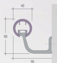
Aluminium mounting bracket
