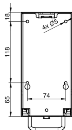
Bohrbild I drilling pattern
