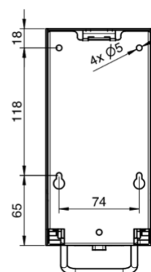
Bohrbild I drilling pattern
